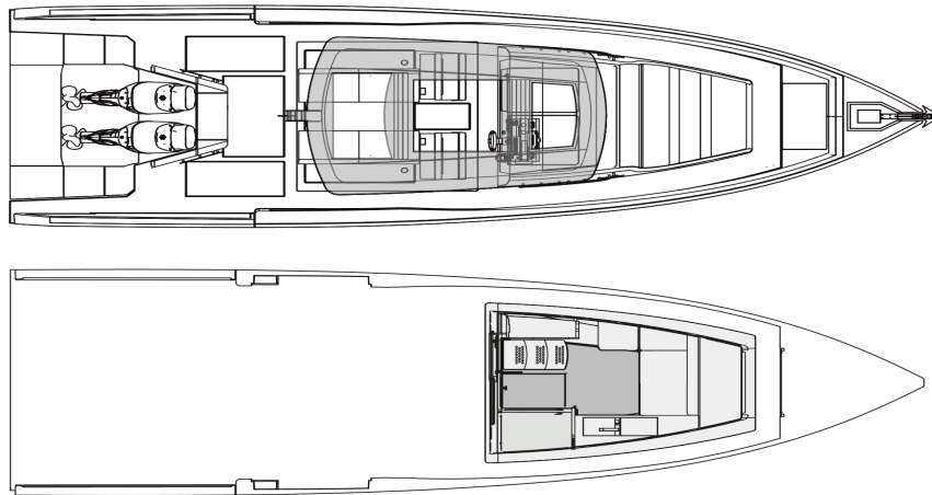
STD layout
